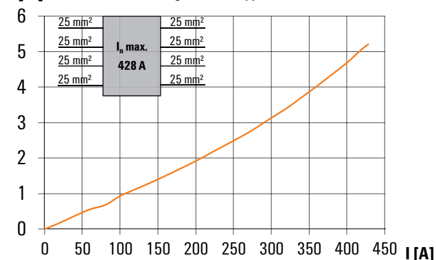
Power loss diagram for copper conductors
